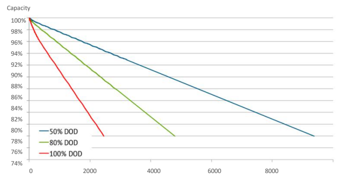
Cycle life in Different DOD @25°C
